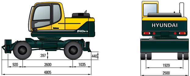
R140W-9 WITH REAR DOZER AND FRONT OUTRIGGER
